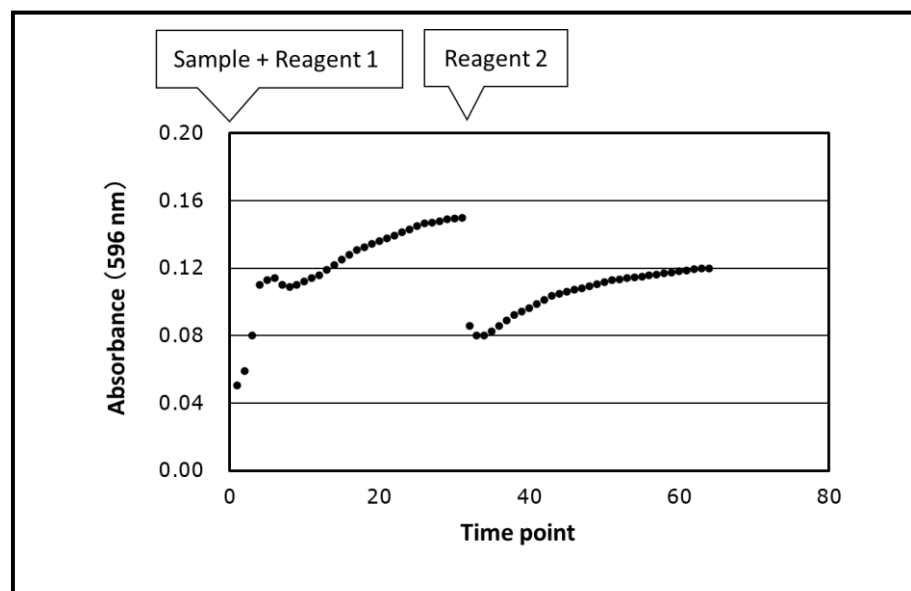
Figure 1: Reaction time course of haptoglobin (1st test)
